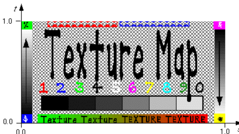
Figure 6.13 -- PixelTexture node
