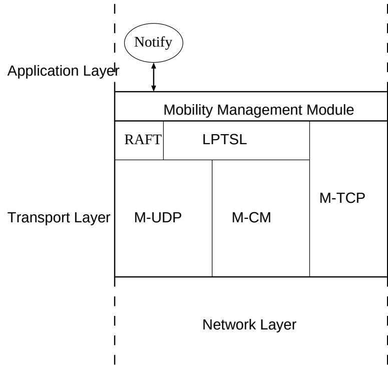
Figure 5: Transport Layer.
