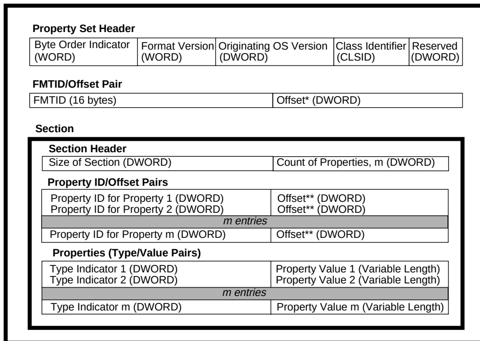
Figure 1. Stream containing a serialized property set
