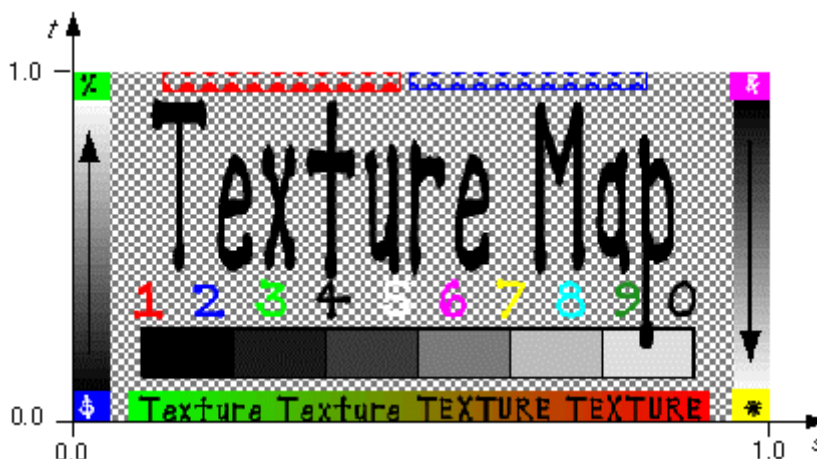
Figure 6.9 -- Texture map coordinate system
