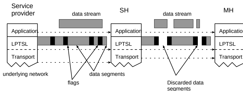
Figure 6: Loss Profile Transport Sub-Layer.
