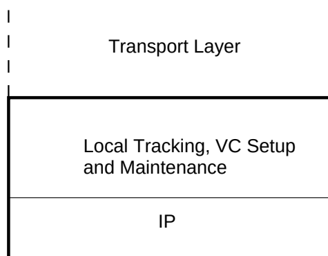
Figure 4: Network Layer.
